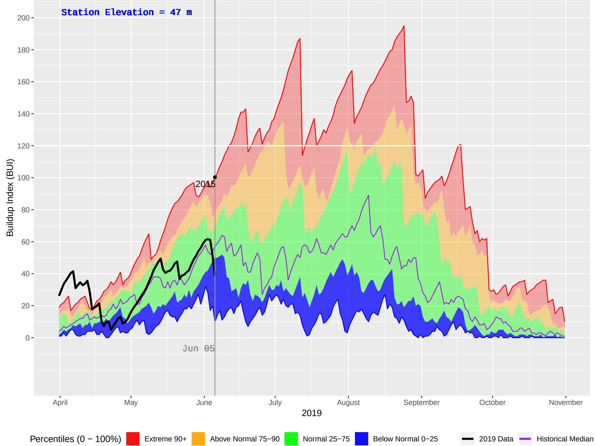
HAGENSBORG 2 (904) : Historical (2005–2018), Current (2019) Daily Buildup Index (BUI)
