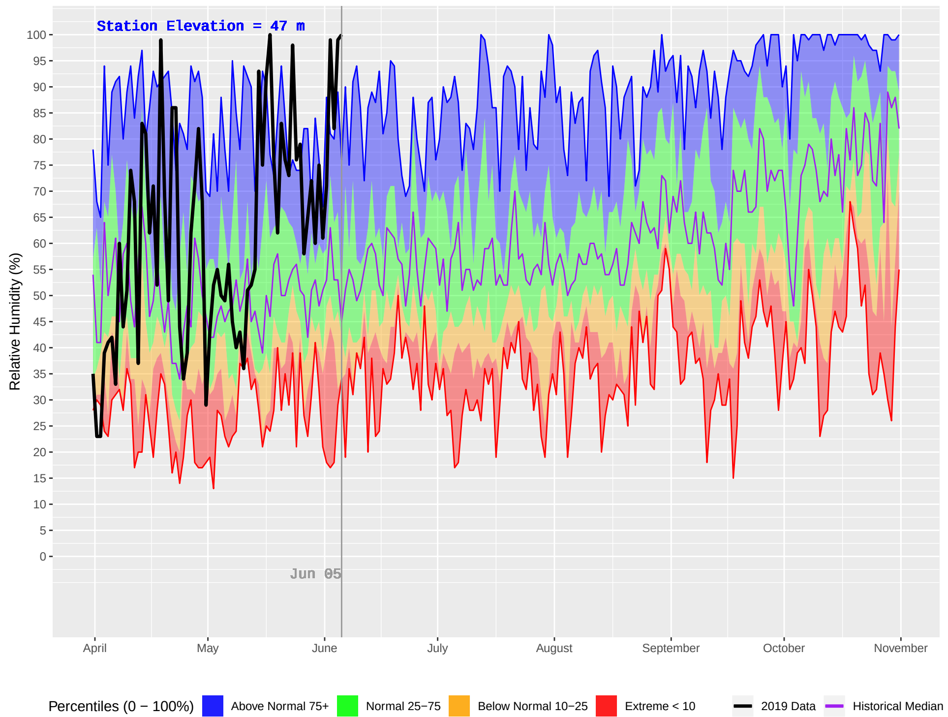
HAGENSBORG 2 (904) : Historical (2005–2018) and Current (2019) Daily Relative Humidity
