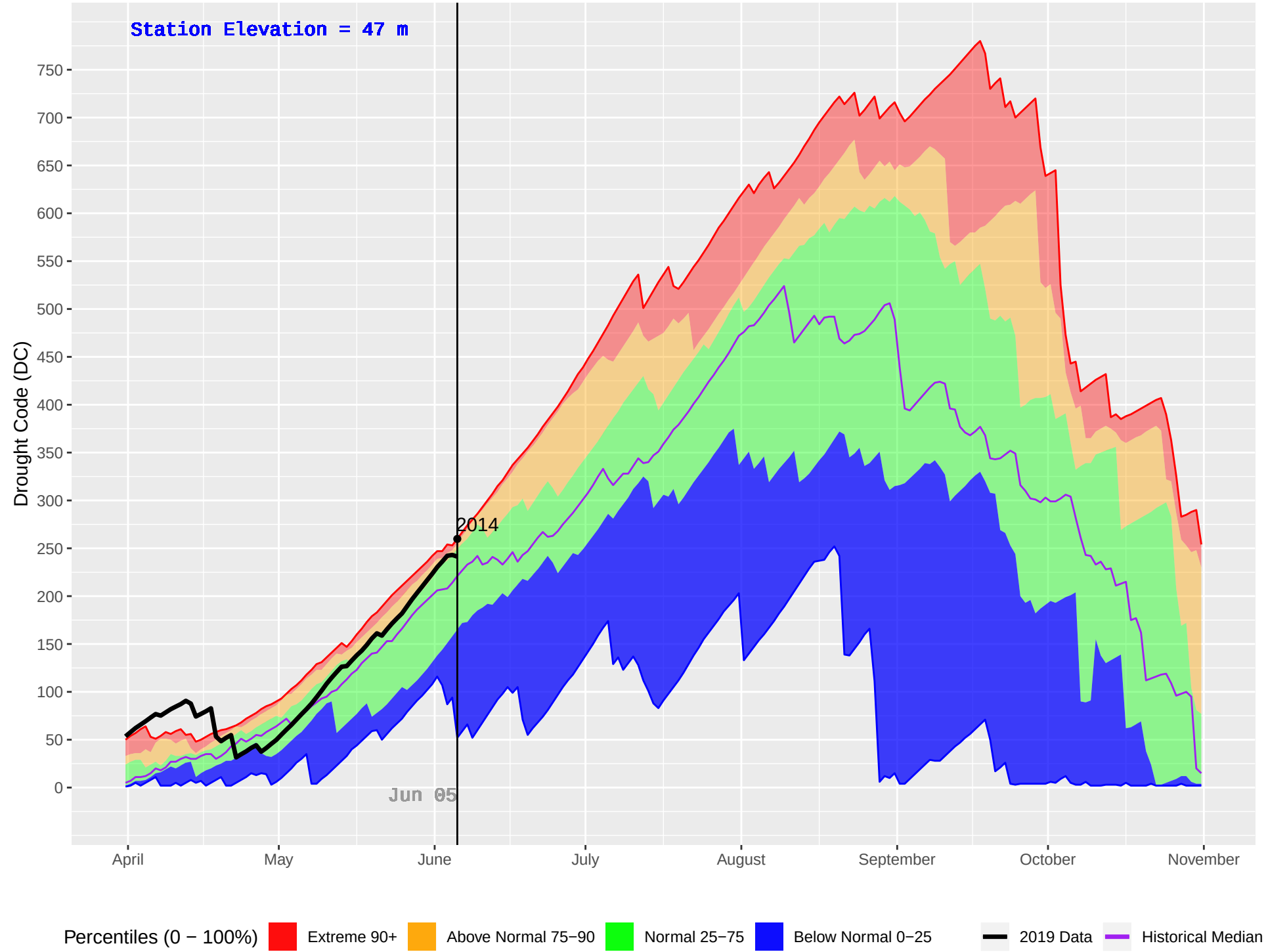
HAGENSBORG 2 (904) : Historical (2005–2018) and Current (2019) Daily Drought Code (DC)
