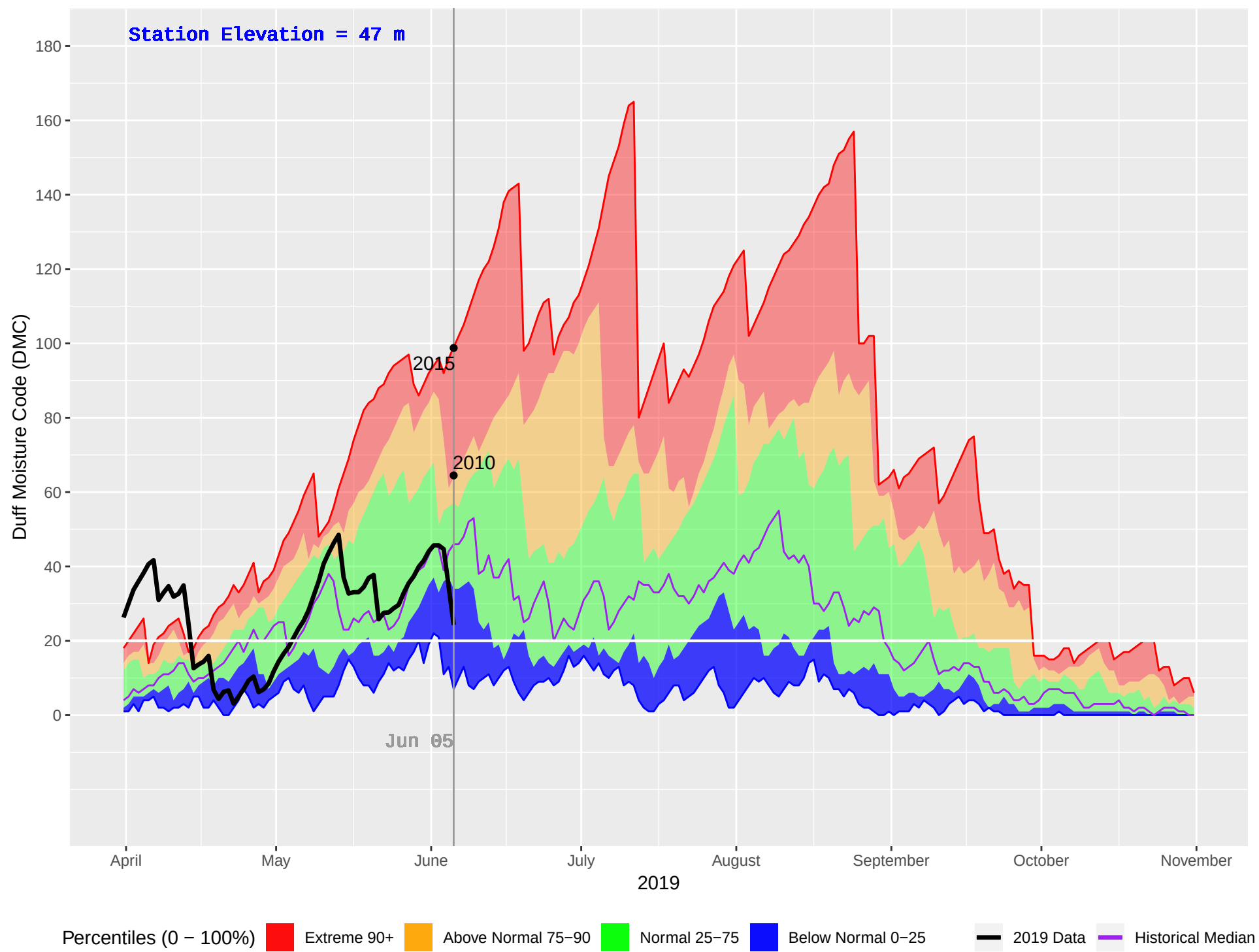
HAGENSBORG 2 (904) : Historical (2005–2018), Current (2019) Daily Duff Moisture Code (DMC)
