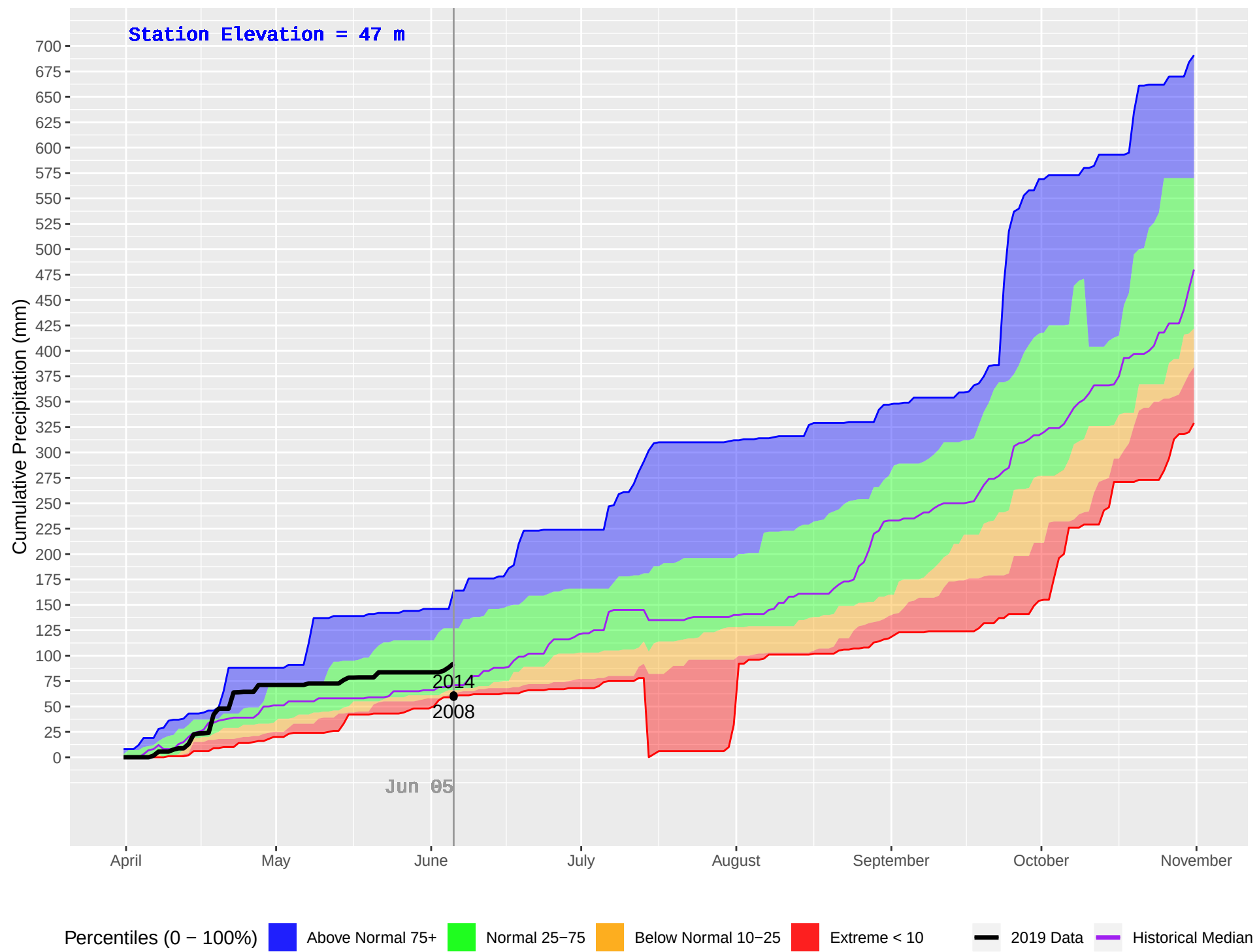
HAGENSBORG 2 (904) : Historical (2005–2018), Current (2019) Daily Cumulative Precipitation
