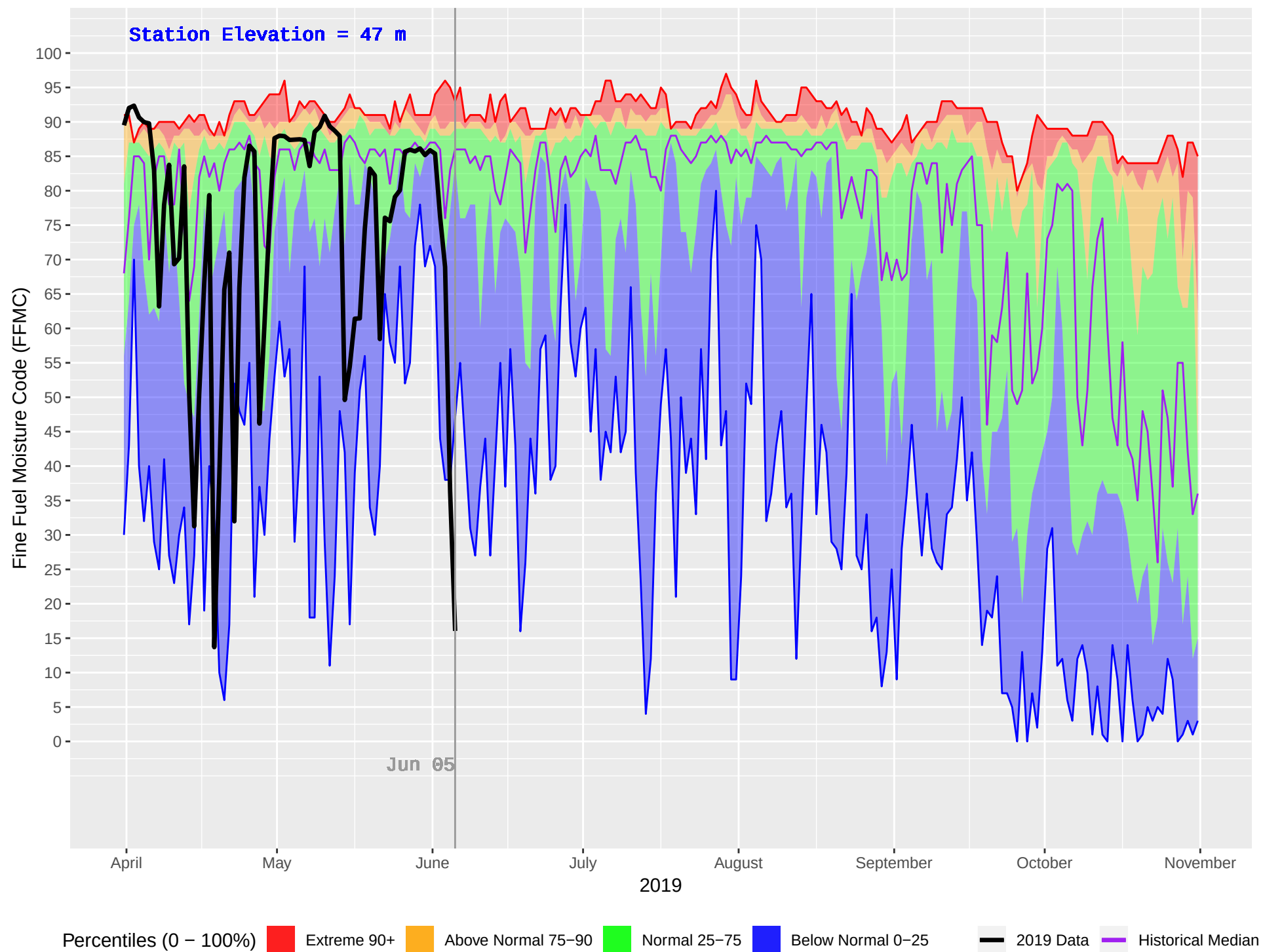
HAGENSBORG 2 (904) : Historical (2005–2018) and Current (2019) Daily Fine Fuel Moisture Code (FFMC)
